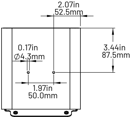
COUNTER MOUNTING PATTERN
